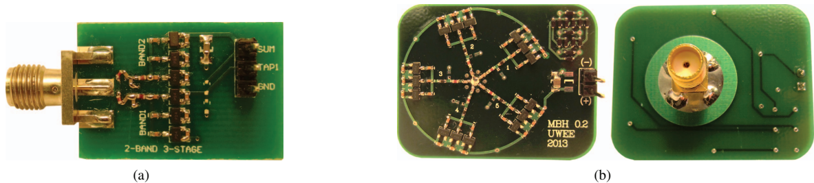
Fig. 8. Two multiband harvester prototypes were constructed: A 2-band harvester (a), and a 5-band harvester with diode summation network (b). The 5-band prototype measures 1.5 by 1.2 inches.
