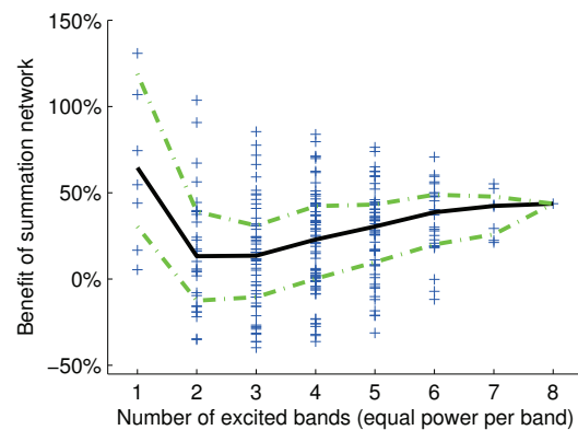
Fig. 7. For the simulated 8-band harvester: Improvement in power output when the diode summation network is used, for every permutation of excited bands. Median and lower and upper quartile of the results are shown.
