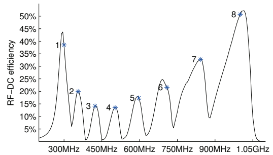
Fig. 5. The RF-DC conversion efficiency of the simulated 8-band harvester, including the diode summation network. Design frequencies for each band are shown.
