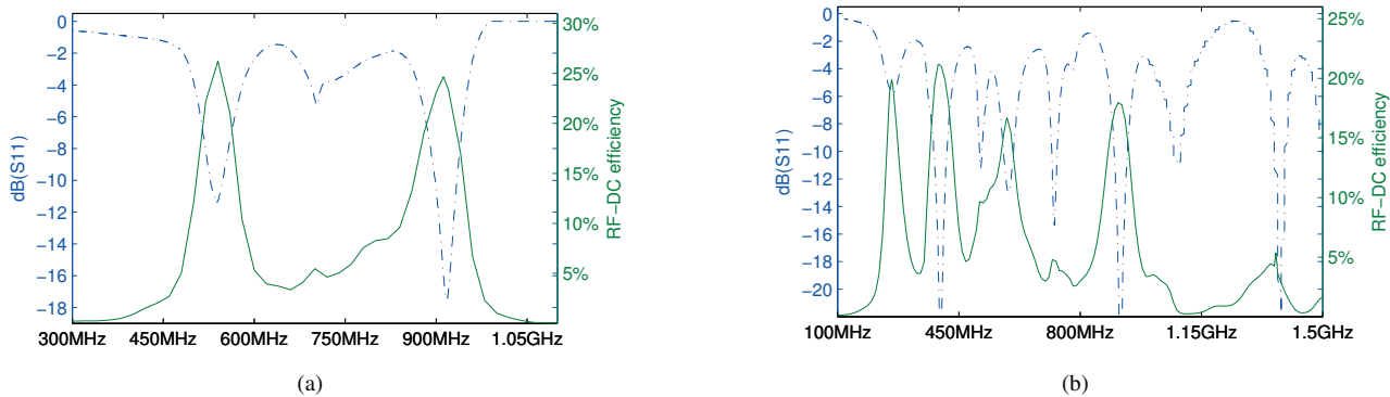
Fig. 9. S11 (reflected power at RF port) and RF-DC conversion efficiency over the operating band for both the 2-band harvester (a) and 5-band harvester (b), for a -10 dBm test power and a 100 k \Omega load.
