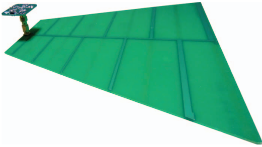
Fig. 11. The 5-band harvester prototype connected to a log-periodic antenna spanning 400-900 MHz.
