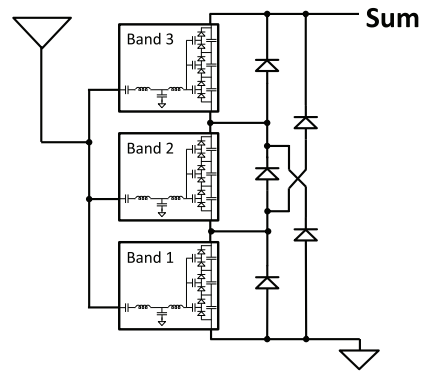
Fig. 4. An example of the summation network, shown here for a 3-band harvester. The output voltage will be the global sum of the band outputs, less a small number of diode drops.
